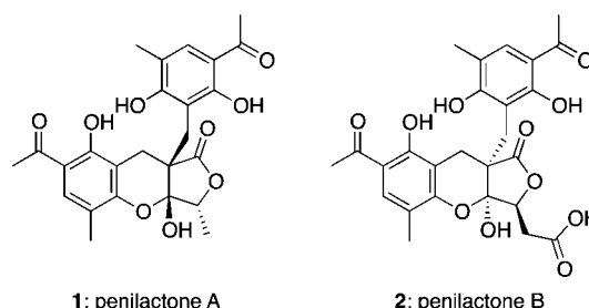
Figure 1. Penilactones A and B.
