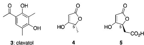
Figure 2. Plausible biosynthetic precursors of the penilactones.
